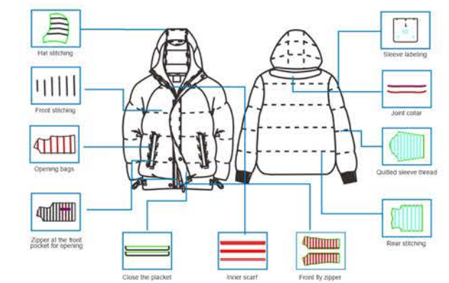
DECOMPOSITION DIAGRAM OF DOWN JACKET PROCESS
